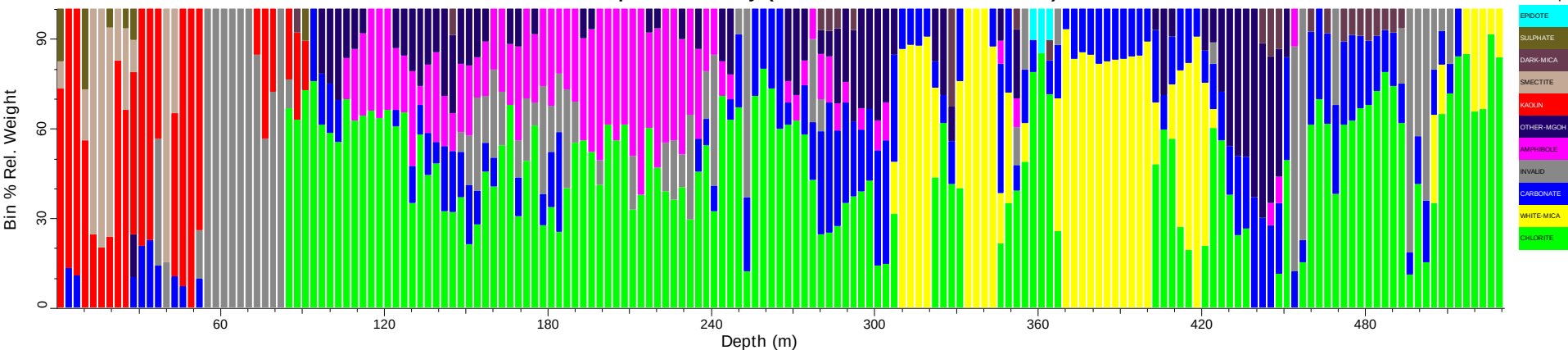
GXDD10_tsg_tir: Spatial Summary (Bin=3 MinBin=5% sjCLST 7.08)
