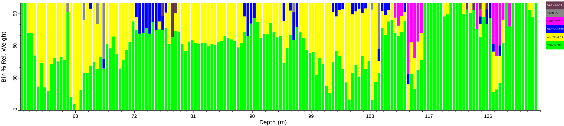
HCRD0047_tsg_tir: Spatial Summary (Bin=0.5 MinBin=5% ujCLST 7.08)
