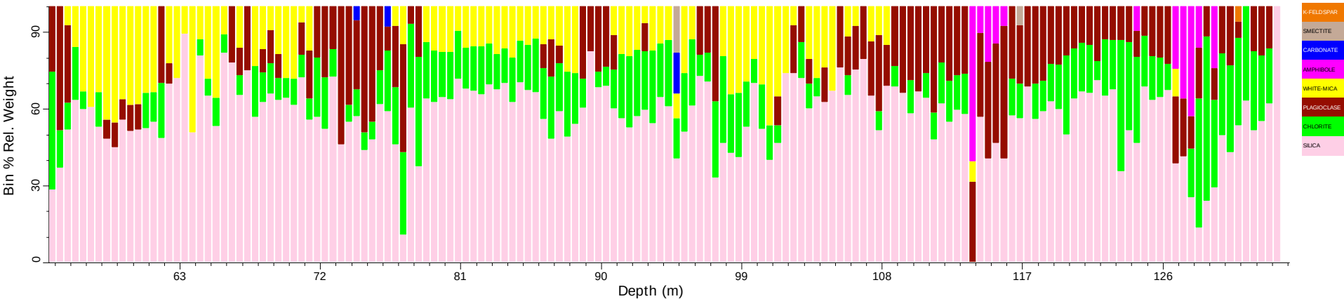
HCRD0047_tsg_tir: Spatial Summary (Bin=0.5 MinBin=5% ujCLST 7.08)
