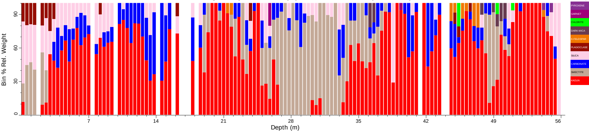
HD009_tsg_tir: Spatial Summary (Bin=0.4 MinBin=5% sjCLST 7.08)
