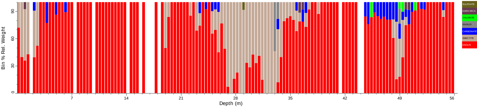
HD009_tsg_tir: Spatial Summary (Bin=0.4 MinBin=5% sjCLST 7.08)
