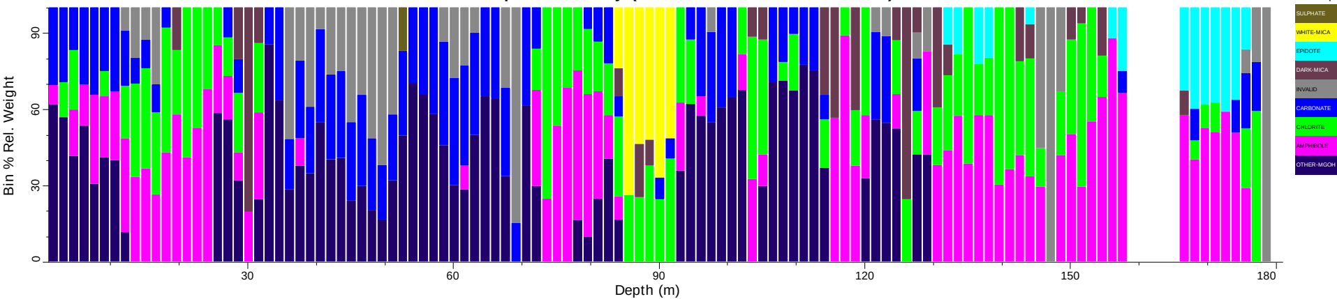
KD1_tsg_tir: Spatial Summary (Bin=1.5 MinBin=5% Set=TIR-CLS1)
