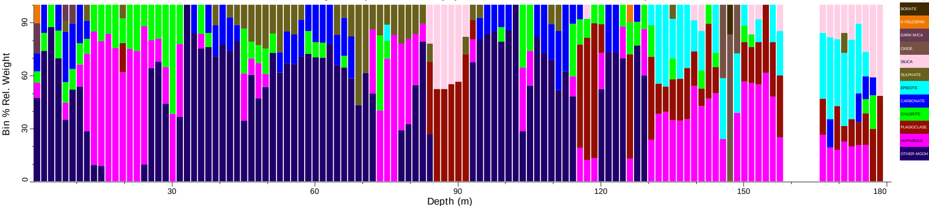
KD1_tsg_tir: Spatial Summary (Bin=1.5 MinBin=5% Set=TIR-CLS1)
