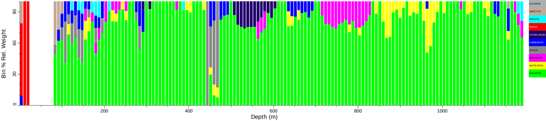
KPDDH009_tsg_tir: Spatial Summary (Bin=8 MinBin=5% sjCLST 7.08)
