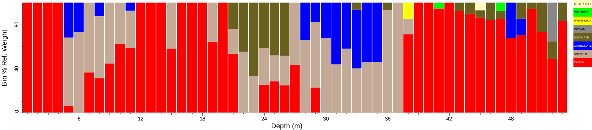
KWAC006_chips_tsg_tir: Spatial Summary (Bin=1 MinBin=5% Un-edited sjCLST 7.08, Mineral Subset)
