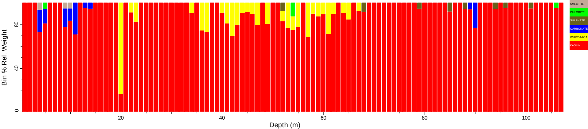
KWAC009_chips_tsg_tir: Spatial Summary (Bin=1 MinBin=5% Un-edited sjCLST 7.08, Mineral Subset)
