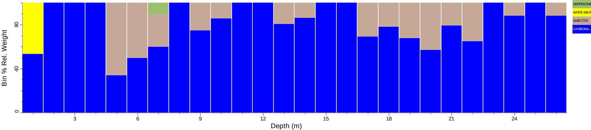
KWAC010_chips_tsg_tir: Spatial Summary (Bin=1 MinBin=5% Un-edited sjCLST 7.08, Mineral Subset)
