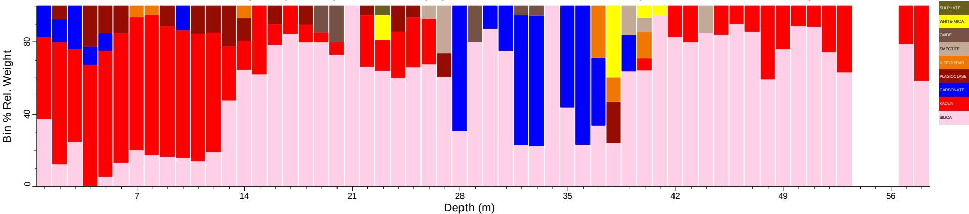
KWAC014_chips_tsg_tir: Spatial Summary (Bin=1 MinBin=5% Un-edited sjCLST 7.08, Mineral Subset)
