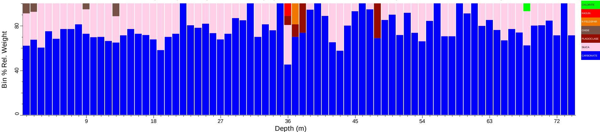
KWAC019_chips_tsg_tir: Spatial Summary (Bin=1 MinBin=5% Un-edited sjCLST 7.08, Mineral Subset)
