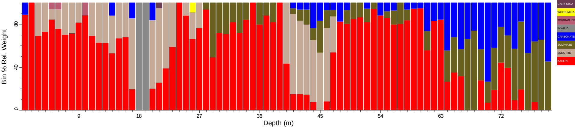
KWAC025_chips_tsg_tir: Spatial Summary (Bin=1 MinBin=5% Un-edited sjCLST 7.08, Mineral Subset)
