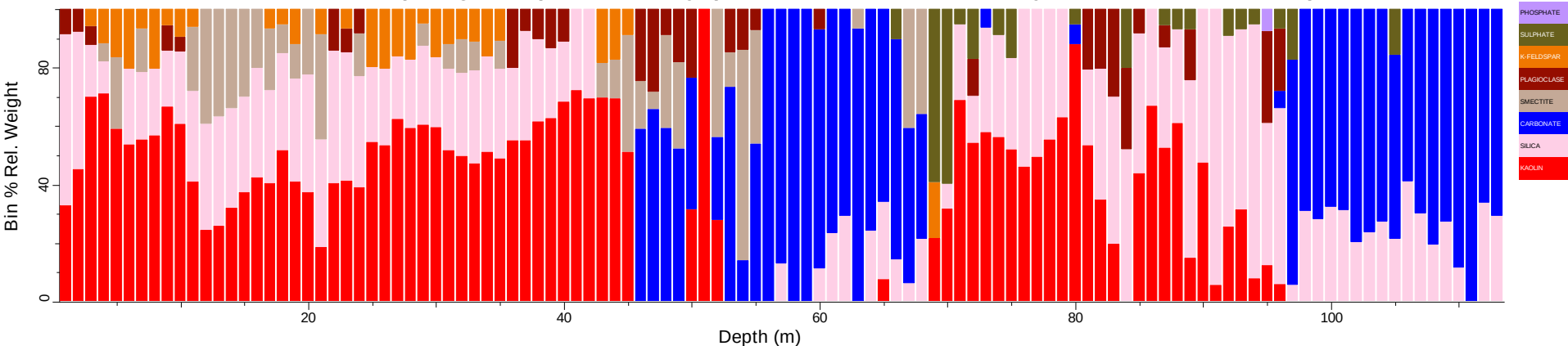
KWAC026_chips_tsg_tir: Spatial Summary (Bin=1 MinBin=5% Un-edited sjCLST 7.08, Mineral Subset)
