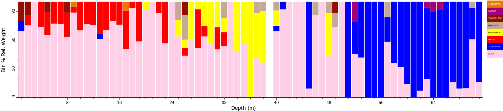
KWAC028_chips_tsg_tir: Spatial Summary (Bin=1 MinBin=5% Un-edited sjCLST 7.08, Mineral Subset)
