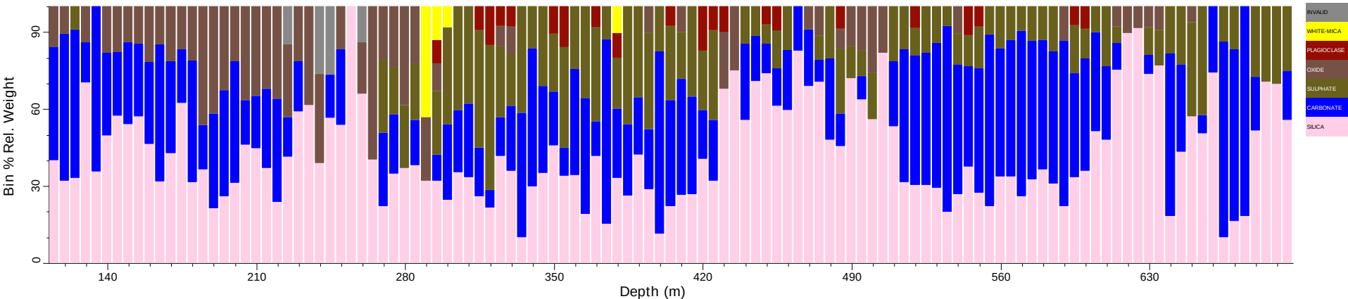
LDDH1_tsg_tir: Spatial Summary (Bin=5 MinBin=5% ujCLST 7.08, Mineral Subset)
