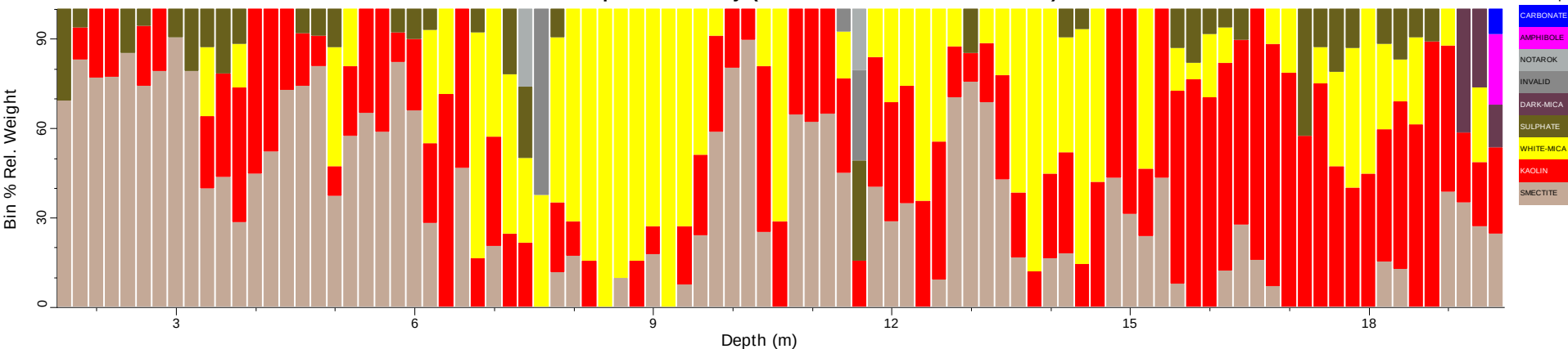
LHD26_tsg_tir: Spatial Summary (Bin=0.2 MinBin=5% sjCLST 7.08)
