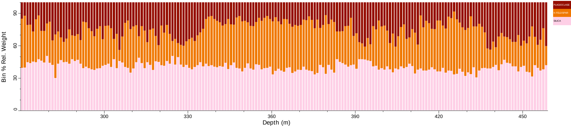
MAD014_tsg_tir: Spatial Summary (Bin=1 MinBin=5% ujCLST 7.08)
