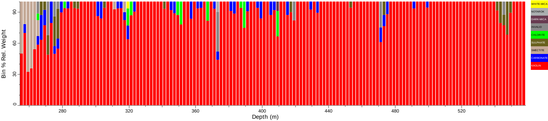
MCH1_tsg_tir: Spatial Summary (Bin=2 MinBin=5% sjCLST 7.08)
