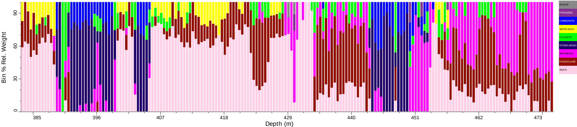
MFED071_tsg_tir: Spatial Summary (Bin=0.5 MinBin=5% ujCLST 7.08)
