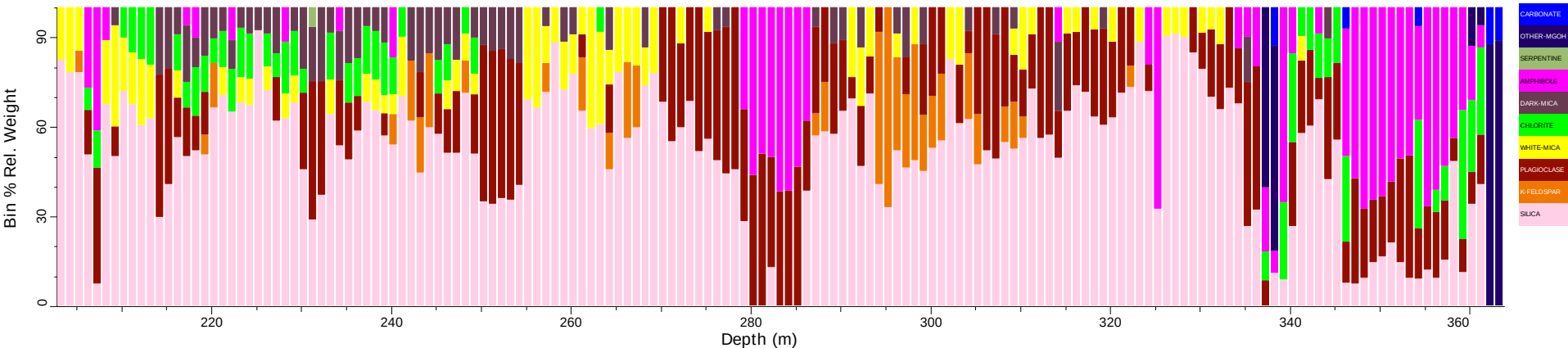
MFED078_tsg_tir: Spatial Summary (Bin=1 MinBin=5% sjCLST 7.08)
