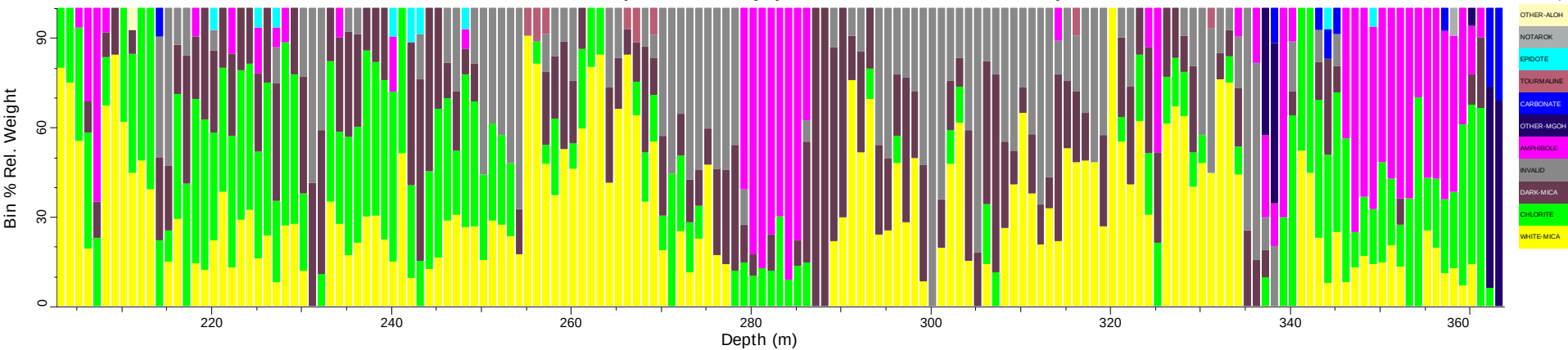
MFED078_tsg_tir: Spatial Summary (Bin=1 MinBin=5% sjCLST 7.08)
