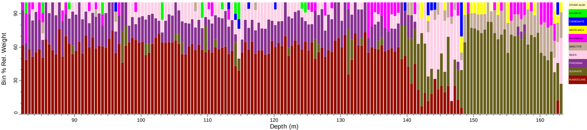
MJGD27_tsg_tir: Spatial Summary (Bin=0.5 MinBin=5% ujCLST 7.08)
