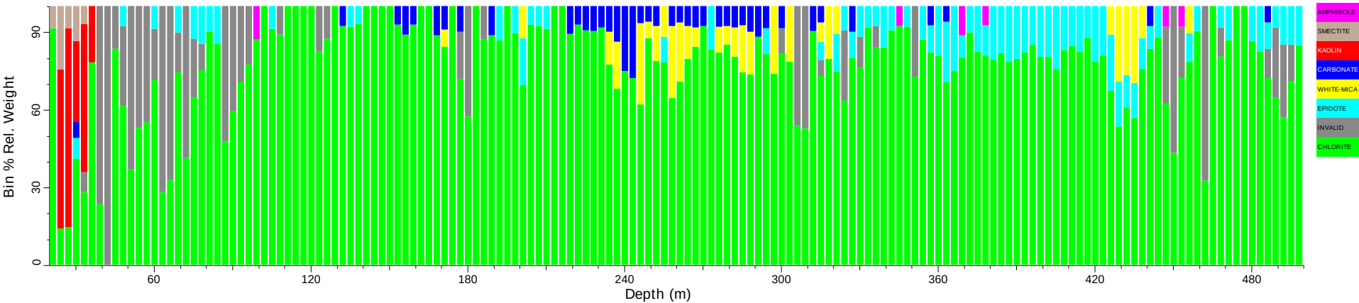
MNDD0004_tsg_tir: Spatial Summary (Bin=3 MinBin=5% ujCLST 7.08)
