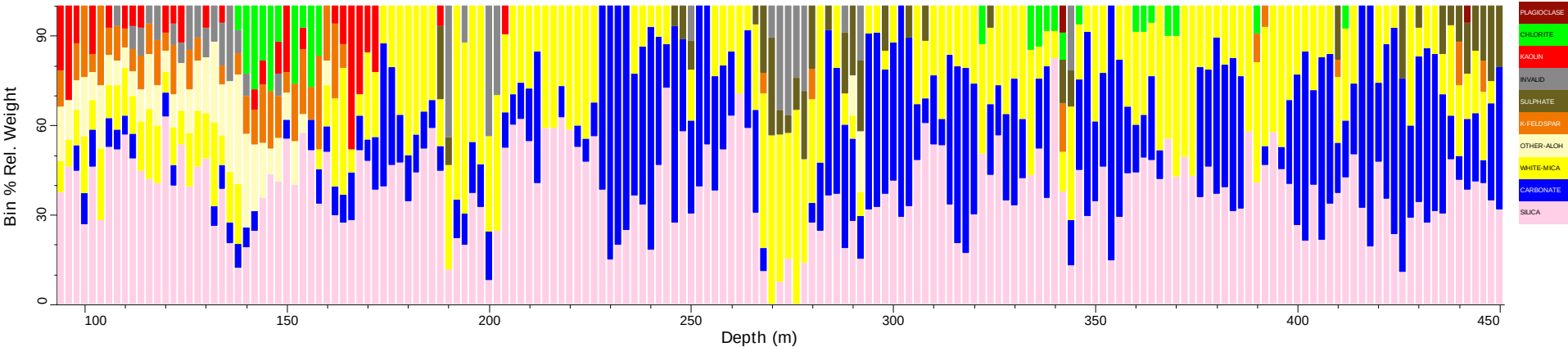
MOD11_tsg_tir: Spatial Summary (Bin=2 MinBin=5% ujCLST 7.08)
