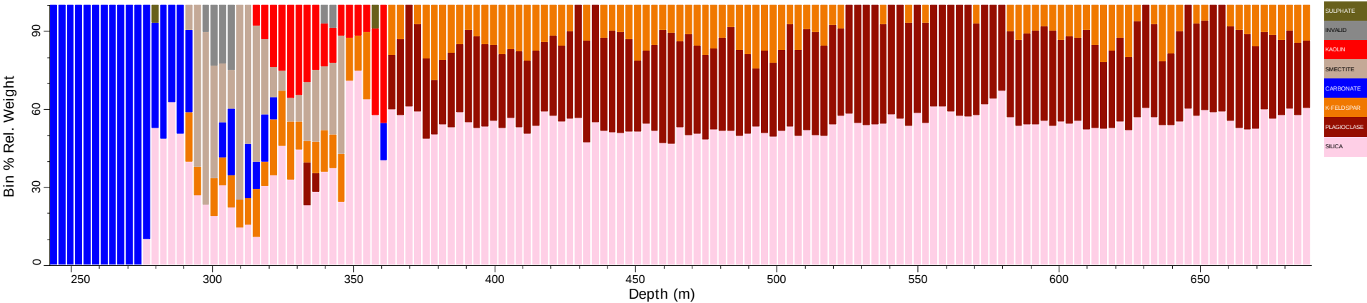
MORCD002_tsg_tir: Spatial Summary (Bin=3 MinBin=5% ujCLST 7.08)
