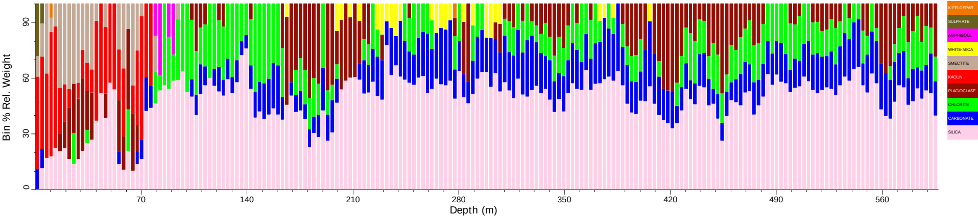
MSD0056_tsg_tir: Spatial Summary (Bin=3 MinBin=5% ujCLST 7.08)
