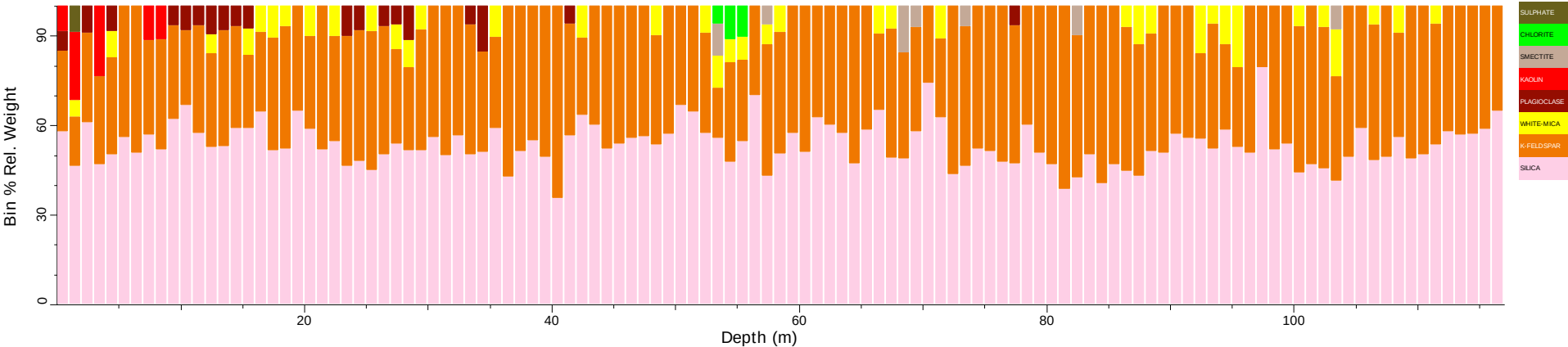
MSD1_tsg_tir: Spatial Summary (Bin=1 MinBin=5% ujCLST 7.08)
