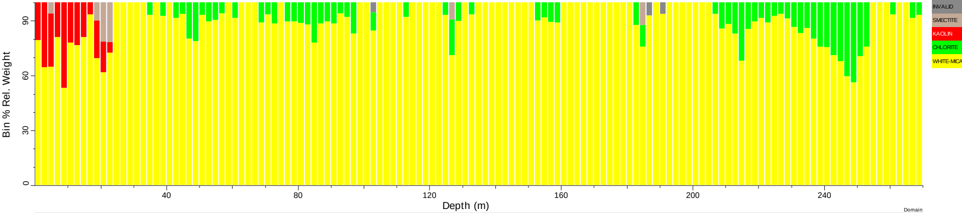
MSD2_tir: Spatial Summary (Bin=2 MinBin=5% ujCLST 7.08)
