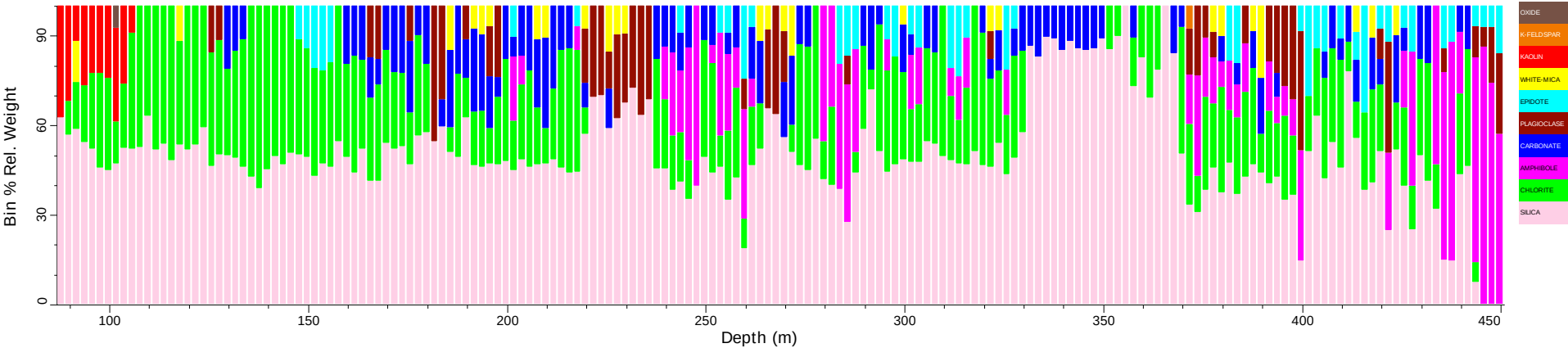
MSDD154_tsg_tir: Spatial Summary (Bin=2 MinBin=5% sjCLST 7.08)
