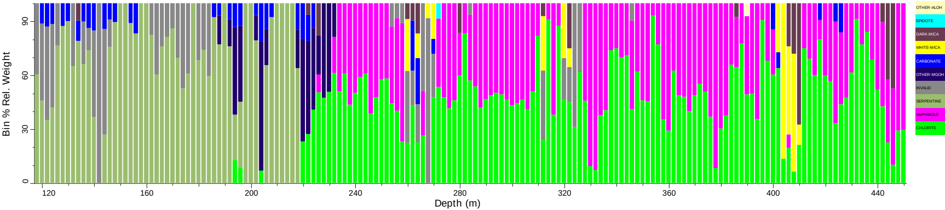
MTD006_tsg_tir: Spatial Summary (Bin=2 MinBin=5% ujCLST 7.08)
