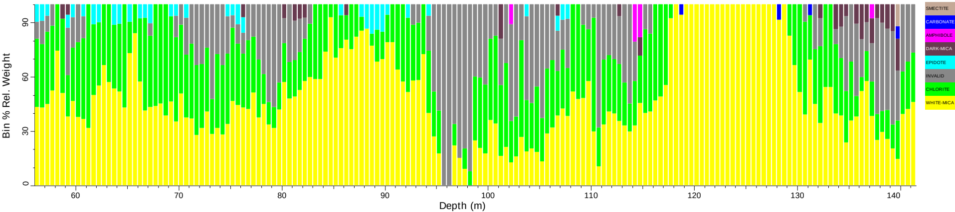
NLD097_tsg_tir: Spatial Summary (Bin=0.5 MinBin=5% ujCLST 7.08)
