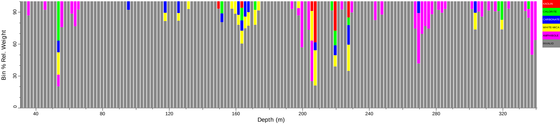
NSD002_tsg_tir: Spatial Summary (Bin=2 MinBin=5% sjCLST 7.08)
