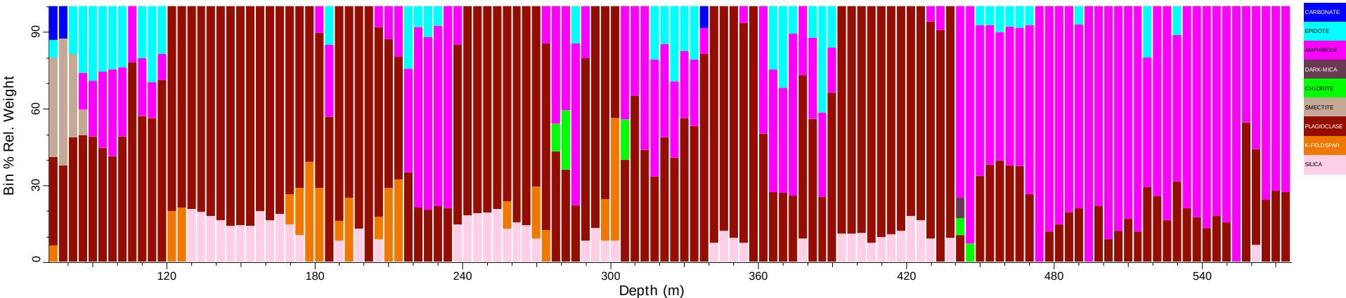
OBUDD003_tsg_tir: Spatial Summary (Bin=4 MinBin=5% sjCLST 7.08)
