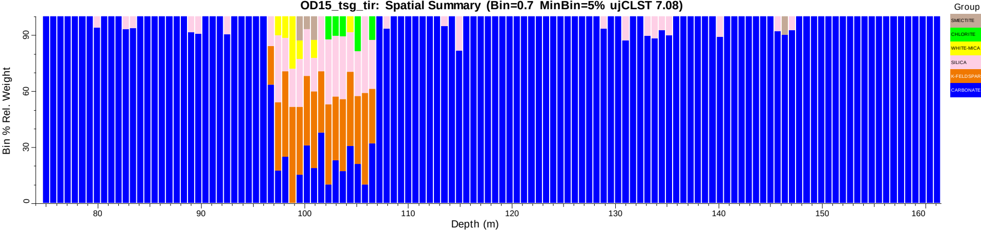
OD15_tsg_tir: Spatial Summary (Bin=0.7 MinBin=5% ujCLST 7.08)
