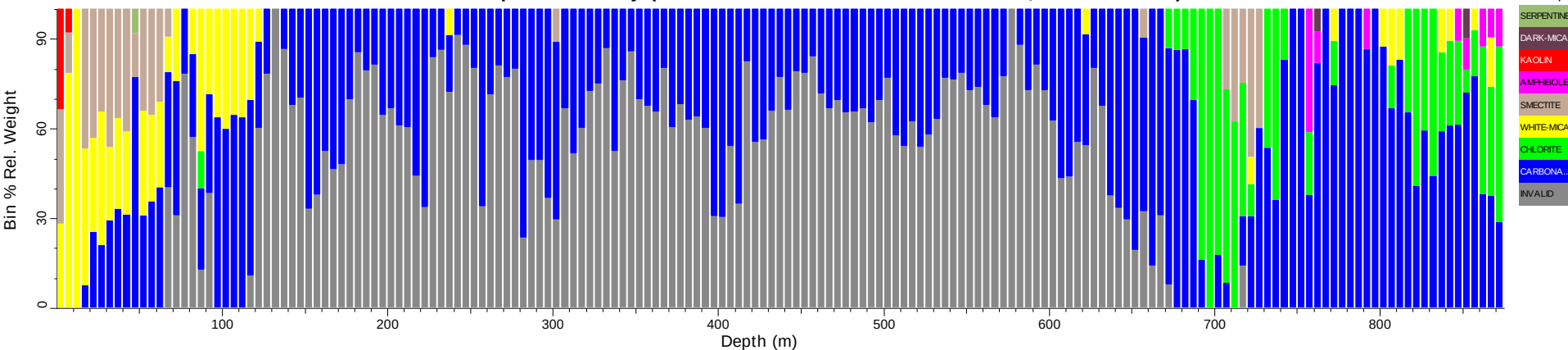
PDD0001_tsg_tir: Spatial Summary (Bin=5 MinBin=5% Un-edited sjCLST 7.08, Mineral Subset)
