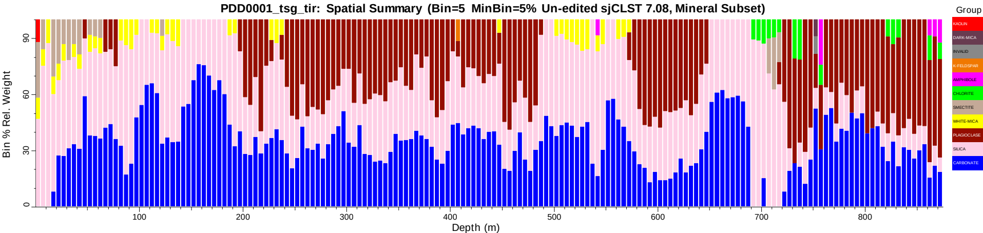
PDD0001_tsg_tir: Spatial Summary (Bin=5 MinBin=5% Un-edited sjCLST 7.08, Mineral Subset)
