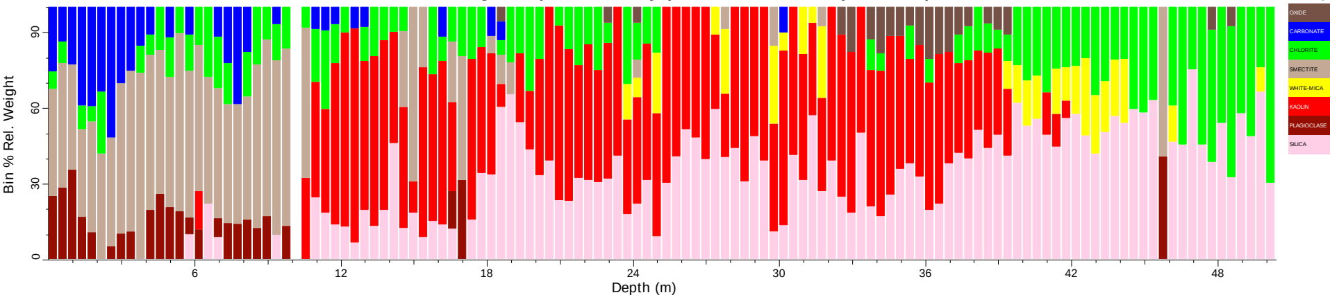
PDP2A_tsg_tir: Spatial Summary (Bin=0.4 MinBin=5% sjCLST 7.08)
