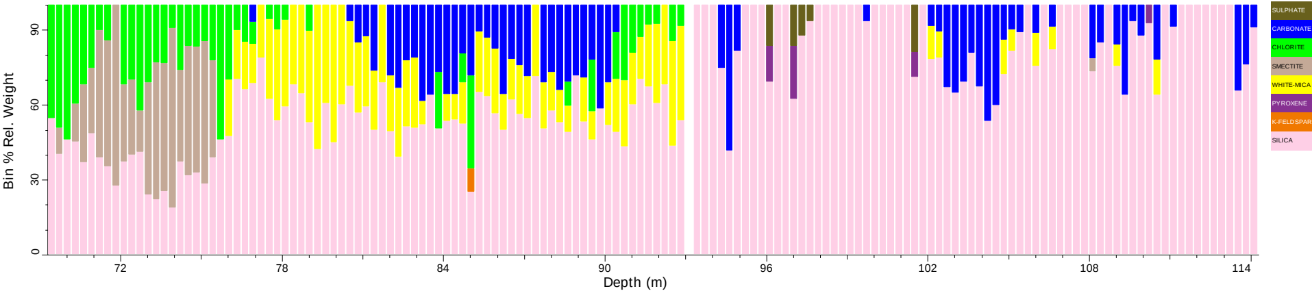
PDP2C_tsg_tir: Spatial Summary (Bin=0.3 MinBin=5% sjCLST 7.08)
