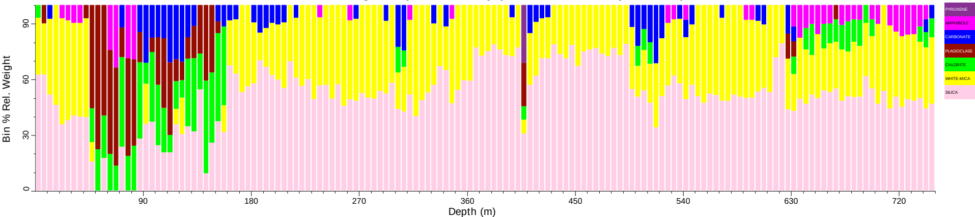
PDU3003_tsg_tir: Spatial Summary (Bin=5 MinBin=5% ujCLST 7.08)
