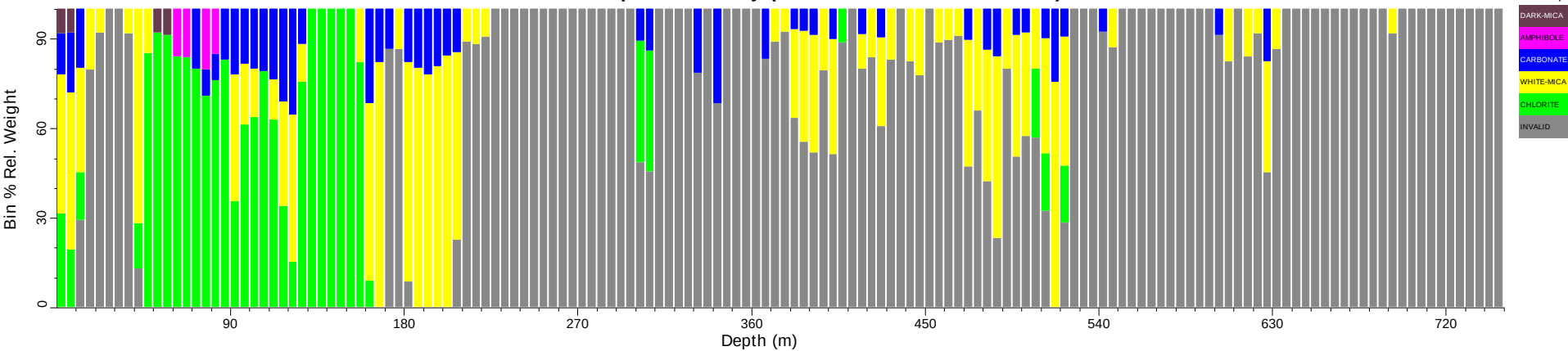
PDU3003_tsg_tir: Spatial Summary (Bin=5 MinBin=5% ujCLST 7.08)
