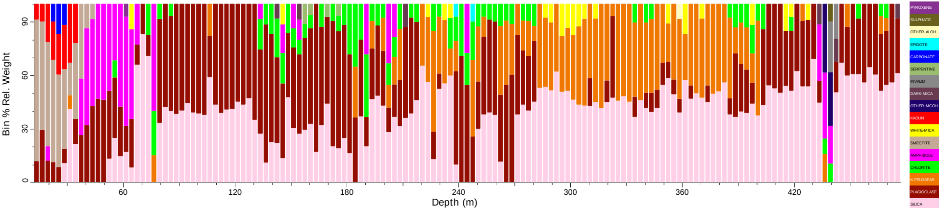
PLJD0002_tsg_tir: Spatial Summary (Bin=3 MinBin=5% sjCLST 7.08)
