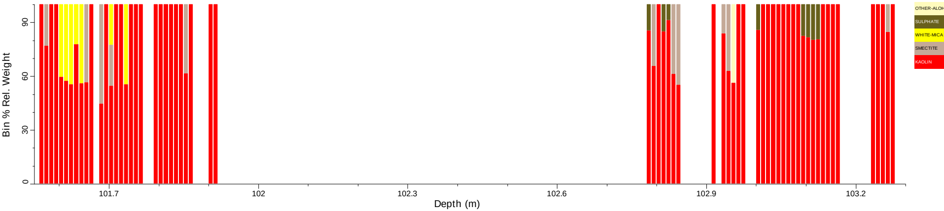
PLWDD005_tsg_tir: Spatial Summary (Bin=0.01 MinBin=5% sjCLST 7.08)
