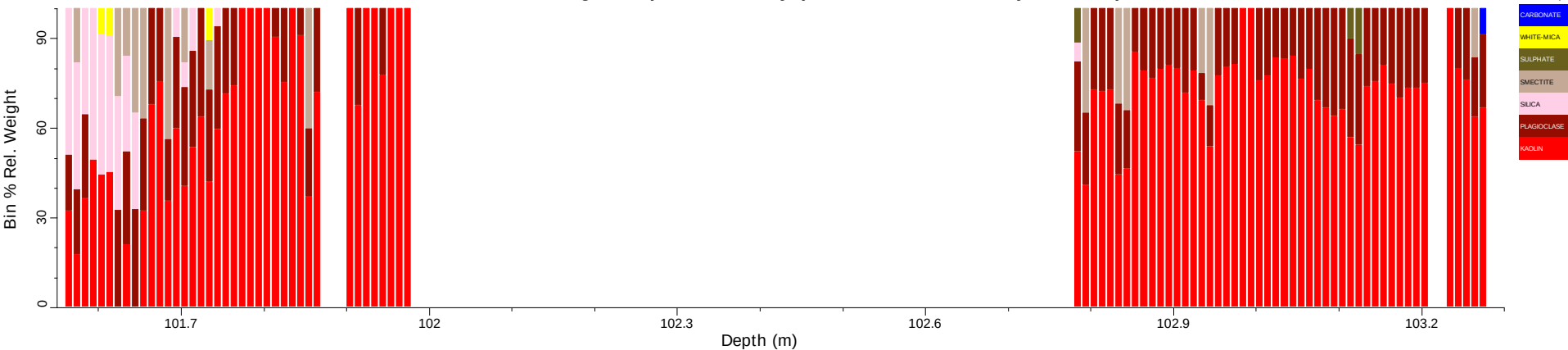
PLWDD005_tsg_tir: Spatial Summary (Bin=0.01 MinBin=5% sjCLST 7.08)
