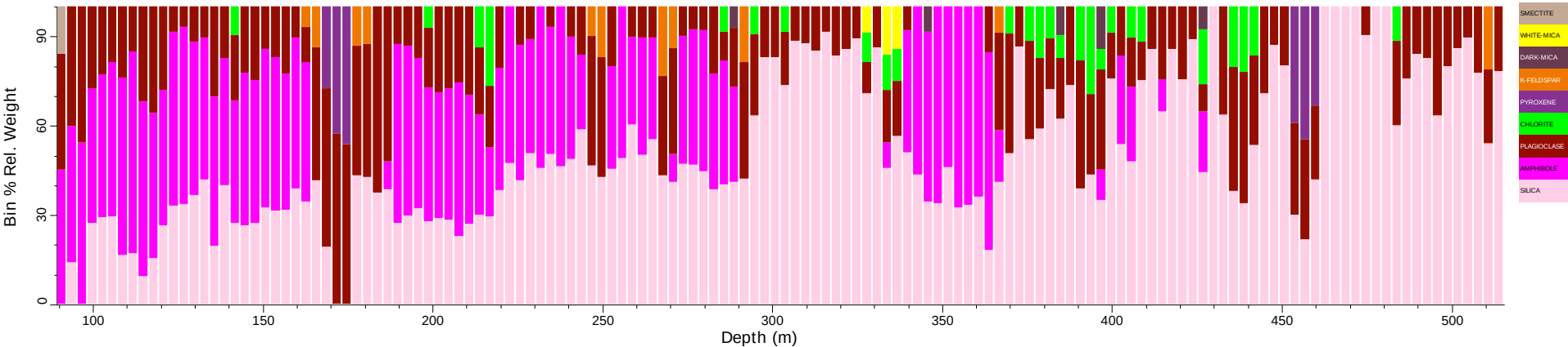
PND002_tsg_tir: Spatial Summary (Bin=3 MinBin=5% ujCLST 7.08)
