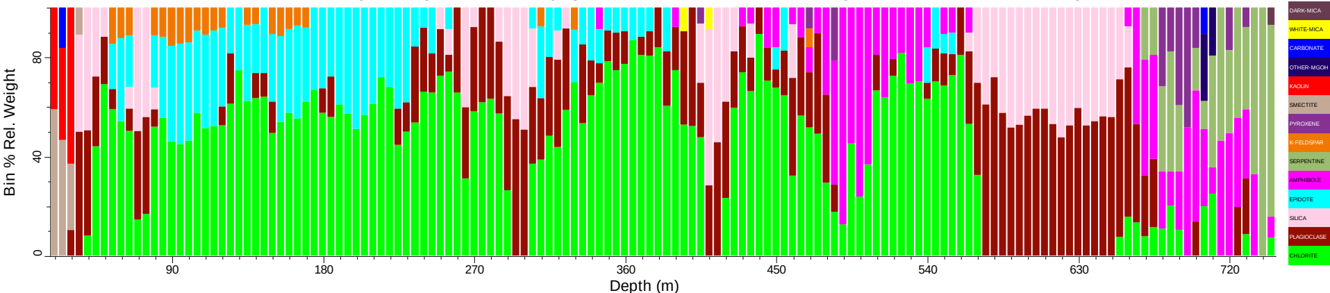
PRDD003_tsg_tir: Spatial Summary (Bin=5 MinBin=5% Un-edited sjCLST 7.08, Mineral Subset)
