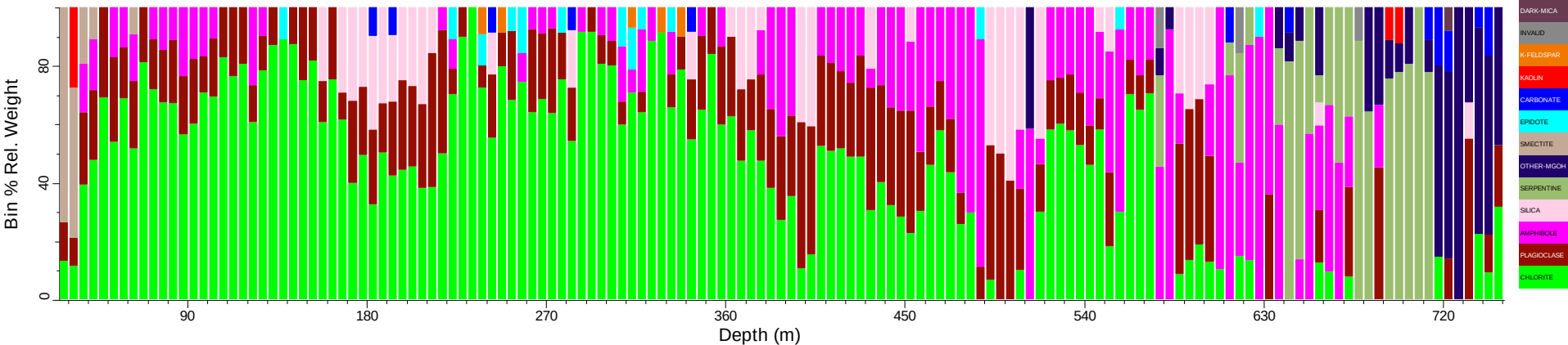
PRDD004_tsg_tir: Spatial Summary (Bin=5 MinBin=5% Un-edited sjCLST 7.08, Mineral Subset)
