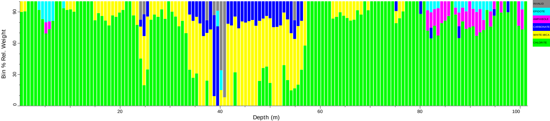
QGCD690_tsg_tir: Spatial Summary (Bin=0.7 MinBin=5% ujCLST 7.08)
