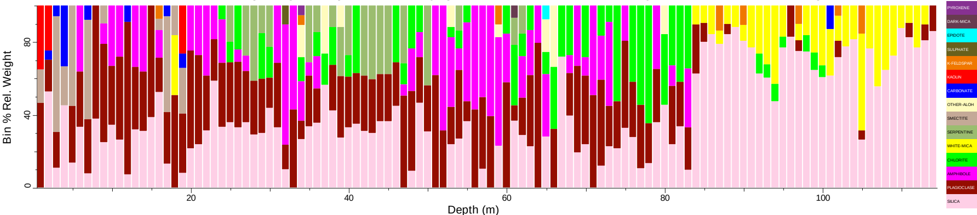
RCRC2201_chips_tsg_tir: Spatial Summary (Bin=1 MinBin=5% Un-edited sjCLST 7.08, Mineral Subset)
