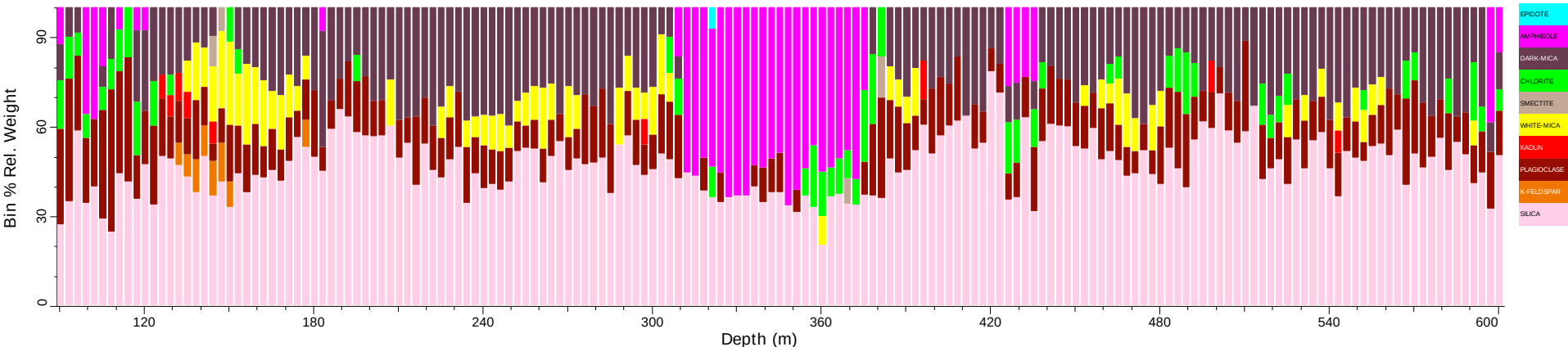
RDH01_tsg_tir: Spatial Summary (Bin=3 MinBin=5% sjCLST 7.08)
