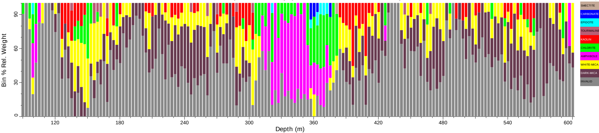
RDH01_tsg_tir: Spatial Summary (Bin=3 MinBin=5% sjCLST 7.08)
