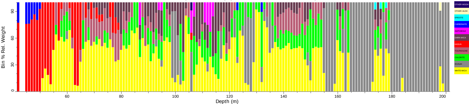
RMSD18_tsg_tir: Spatial Summary (Bin=1 MinBin=5% sjCLST 7.08)
