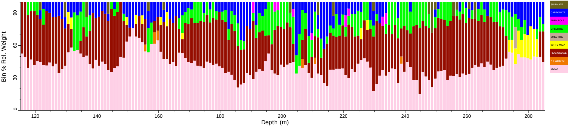
ROAD002_tsg_tir: Spatial Summary (Bin=1 MinBin=5% sjCLST 7.08)
