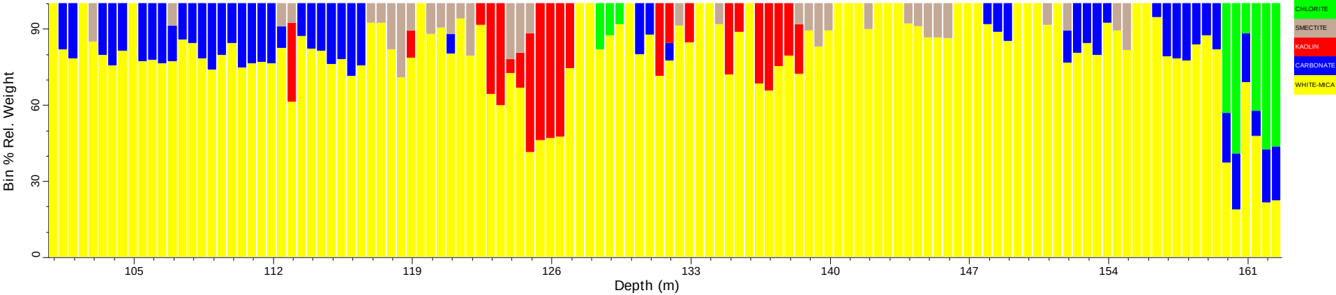
ROAD006_tsg_tir: Spatial Summary (Bin=0.5 MinBin=5% sjCLST 7.08)
