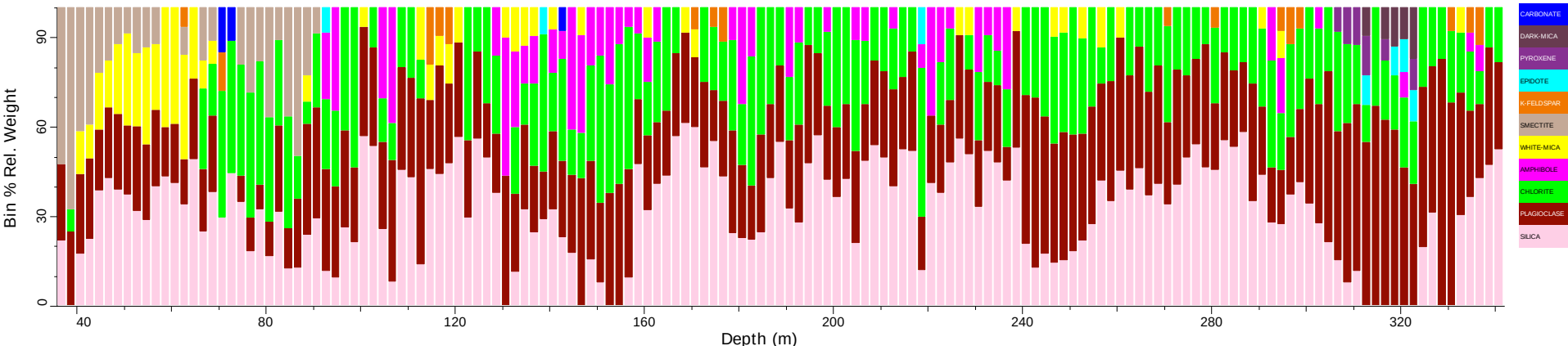
RUD0003_tir: Spatial Summary (Bin=2 MinBin=5% sjCLST 7.08)
