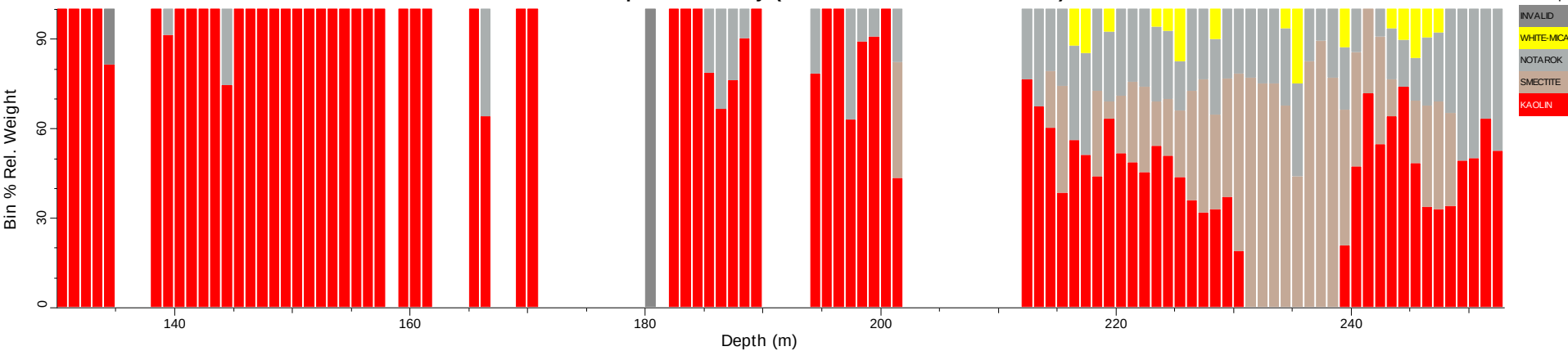
SC000021_tsg_tir: Spatial Summary (Bin=1 MinBin=5% sjCLST 7.08)
