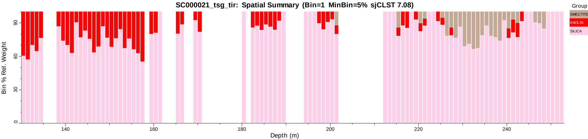
SC000021_tsg_tir: Spatial Summary (Bin=1 MinBin=5% sjCLST 7.08)
