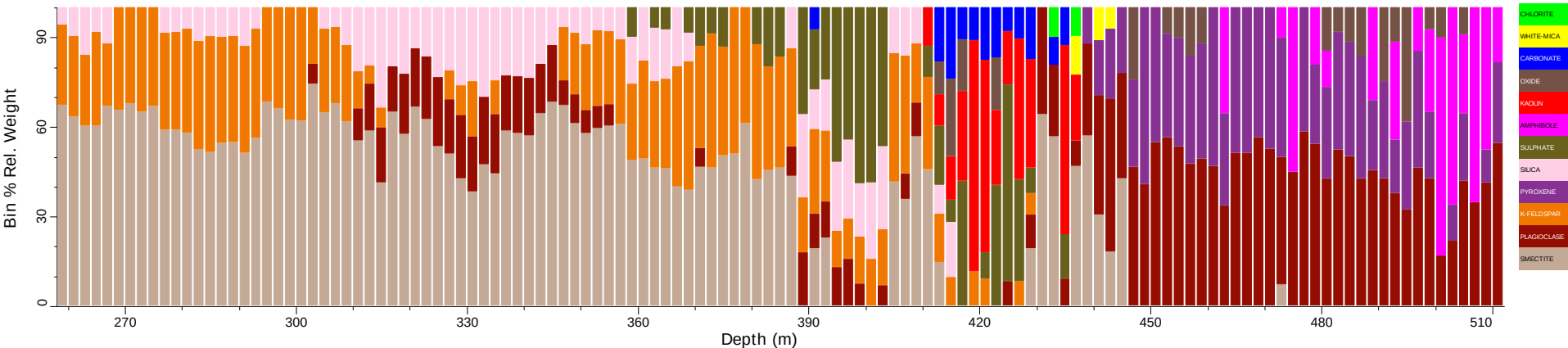
SDDH2_tsg_tir: Spatial Summary (Bin=2 MinBin=5% ujCLST 7.08)
